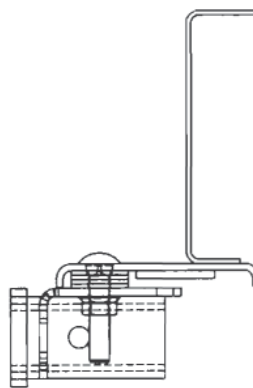
FORD BUMPER STYLE 2
